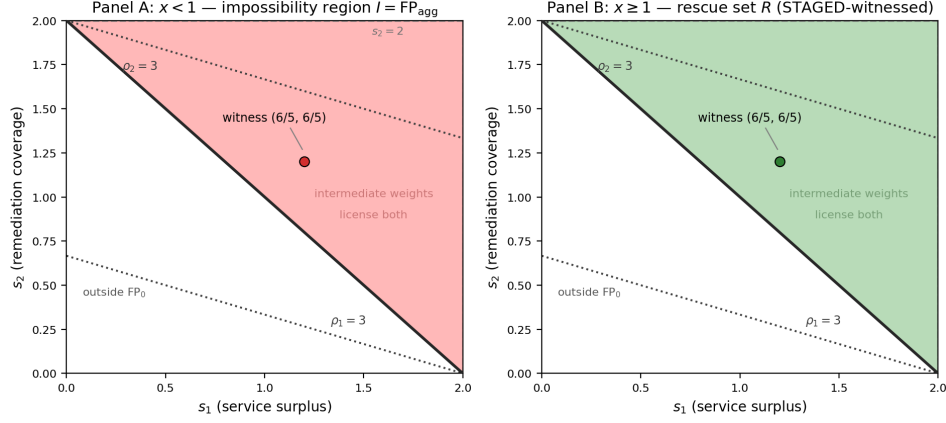
Figure 1: The discrepancy region \mathcal{Q} in the floor plane: the closed upper-right triangle above s_1 + s_2 = 2 , minus the legs s_1 = 2 and s_2 = 2 (boundary conventions as in Section 4.6). Panel A ( x < 1 , shown at x = 0 ): \mathcal{Q} is the impossibility region I = \text{FP}_{\text{agg}} , with the interior witness (s_1, s_2) = (6/5, 6/5) marked. Panel B ( x \geq 1 , shown at x = 1 ): the same region is the rescue set R , served by STAGED. The threshold curves \rho_1, \rho_2 bound the FAST-only / both / SLOW-only endorsement zones; the point (x, s_1, s_2) = (\frac{1}{2}, \frac{1}{10}, \frac{1}{10}) , outside the s -plane section, is annotated in Panel A.
